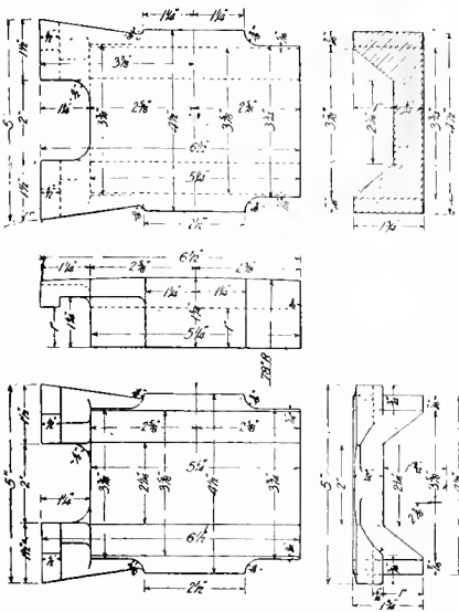
Figs. 5389-5393. WEDGE.
